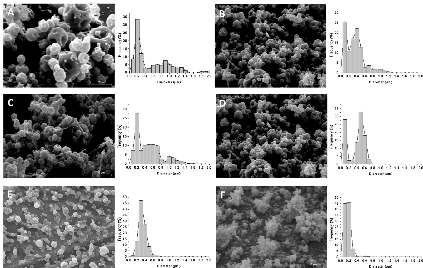
Fig. 1. Selected SEM images and their corresponding capsule size distribution of resistant starch-based structures with the different surfactants: (A) 5% Span20; (B) 30% Span20; (C) 5% Tween20; (D) 30% Tween20; (E) 5% lecithin and (F) 30% lecithin.
