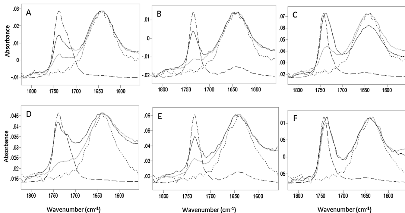
Fig. 4. ATR-FTIR spectra from 1800 to 1600 \text{cm}^{-1} for the pure carbohydrate (dotted line), the surfactants (dashed line), the carbohydrate with 5% of surfactant (gray line) and with 30% of surfactant (black line) for: (A) resistant starch/Span20; (B) resistant starch/Tween20; (C) resistant starch/lecithin; (D) maltodextrin/Span20; (E) maltodextrin/Tween20; and (F) maltodextrin/lecithin (F).
