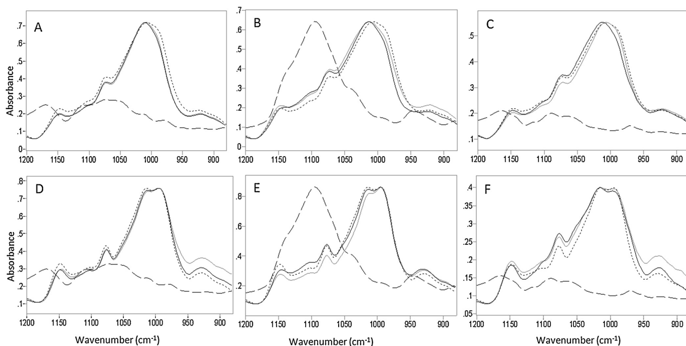
Fig. 3. ATR-FTIR spectra from 1200 to 880 \text{cm}^{-1} for the pure carbohydrate (dotted line), the surfactants (dashed line), the carbohydrate with 5% of surfactant (gray line) and with 30% of surfactant (black line) for: (A) resistant starch/Span20; (B) resistant starch/Tween20; (C) resistant starch/lecithin; (D) maltodextrin/Span20; (E) maltodextrin/Tween20; and (F) maltodextrin/lecithin.
